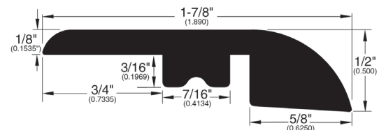
297 - Overlap Reducer
