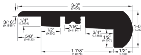
288 - Flush/Overlap Stair Nosing
