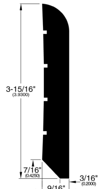
294 - Wall Base
