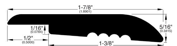
297 - Overlap Reducer
