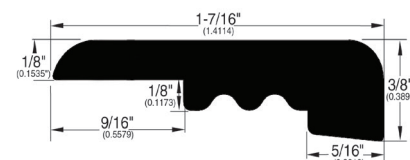
290 - Overlap Reducer
